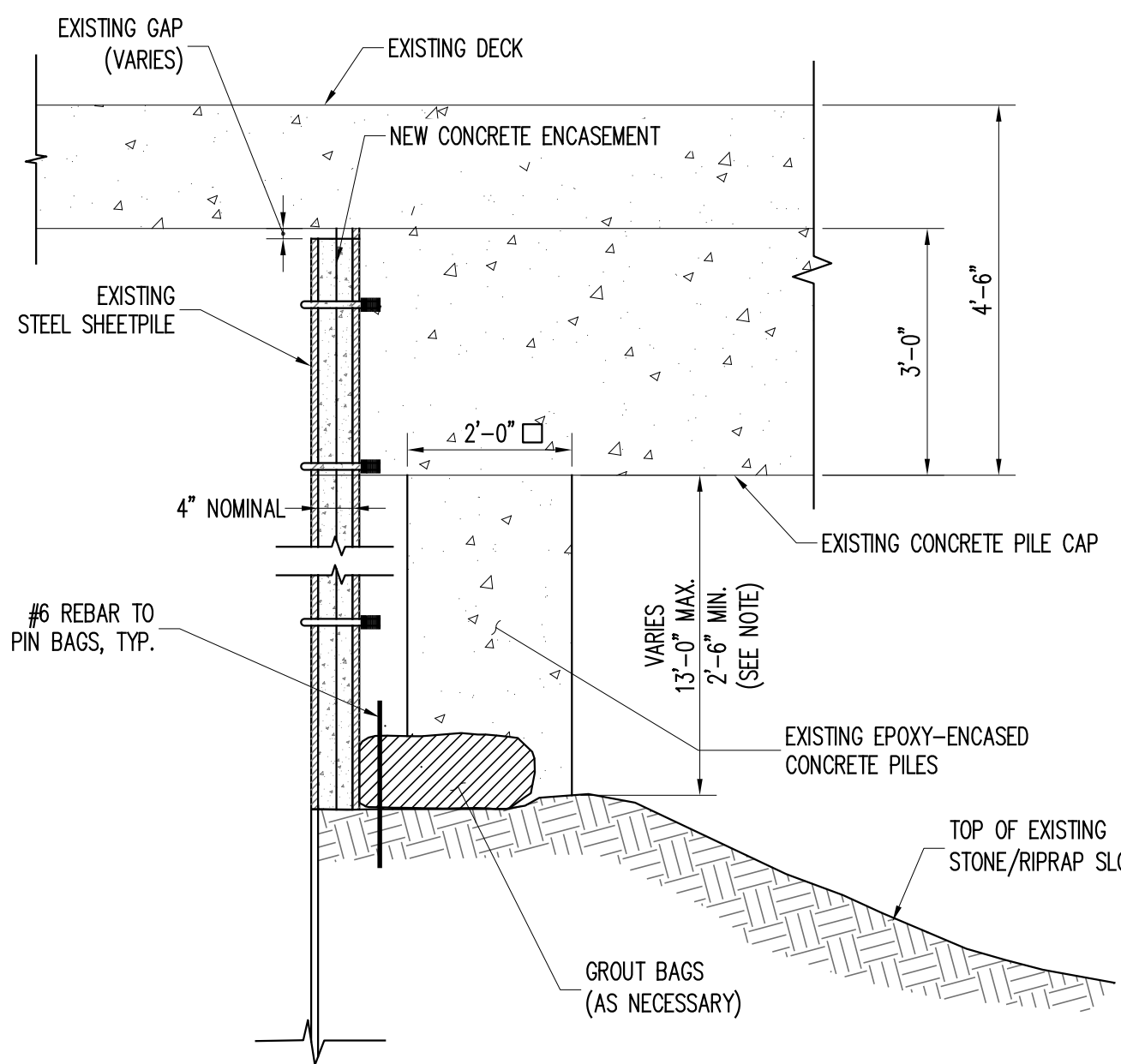
C TYPICAL SECTION THROUGH ENCASEMENT S-140 SCALE: 1/2" = 1'-0" FEET NOTE: FOR DISTANCE FROM BOTTOM OF PILE CAP TO MUDLINE, SEE TABLE ON S-120
