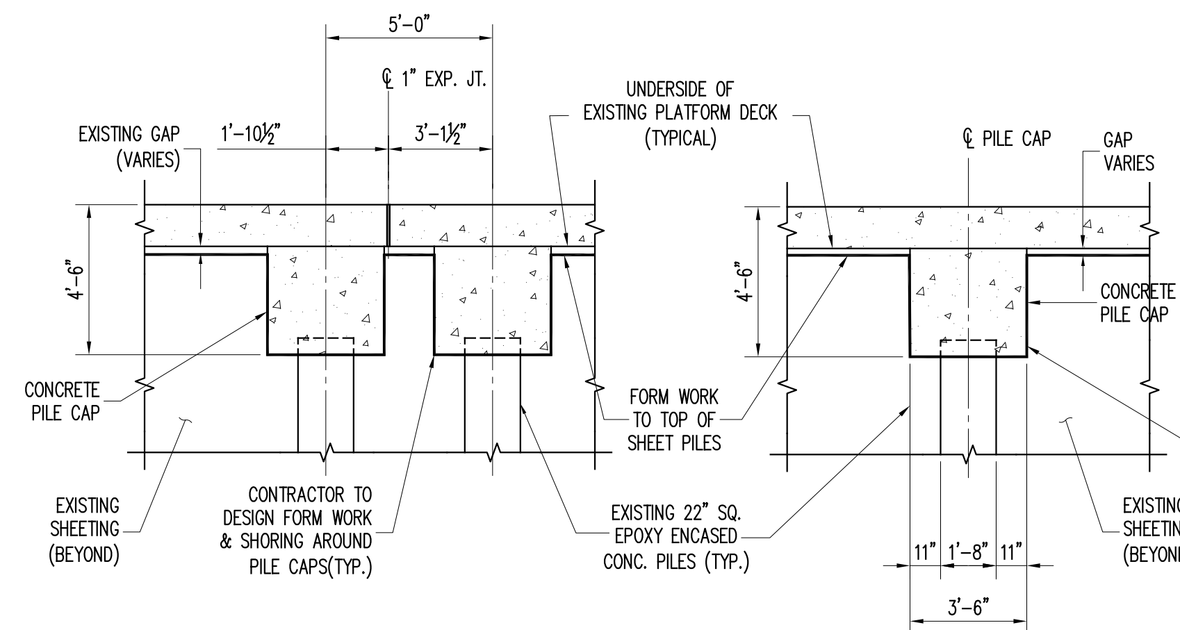
D PILE CAP SECTION S-140 SCALE: 1/4" = 1'-0" FEET
