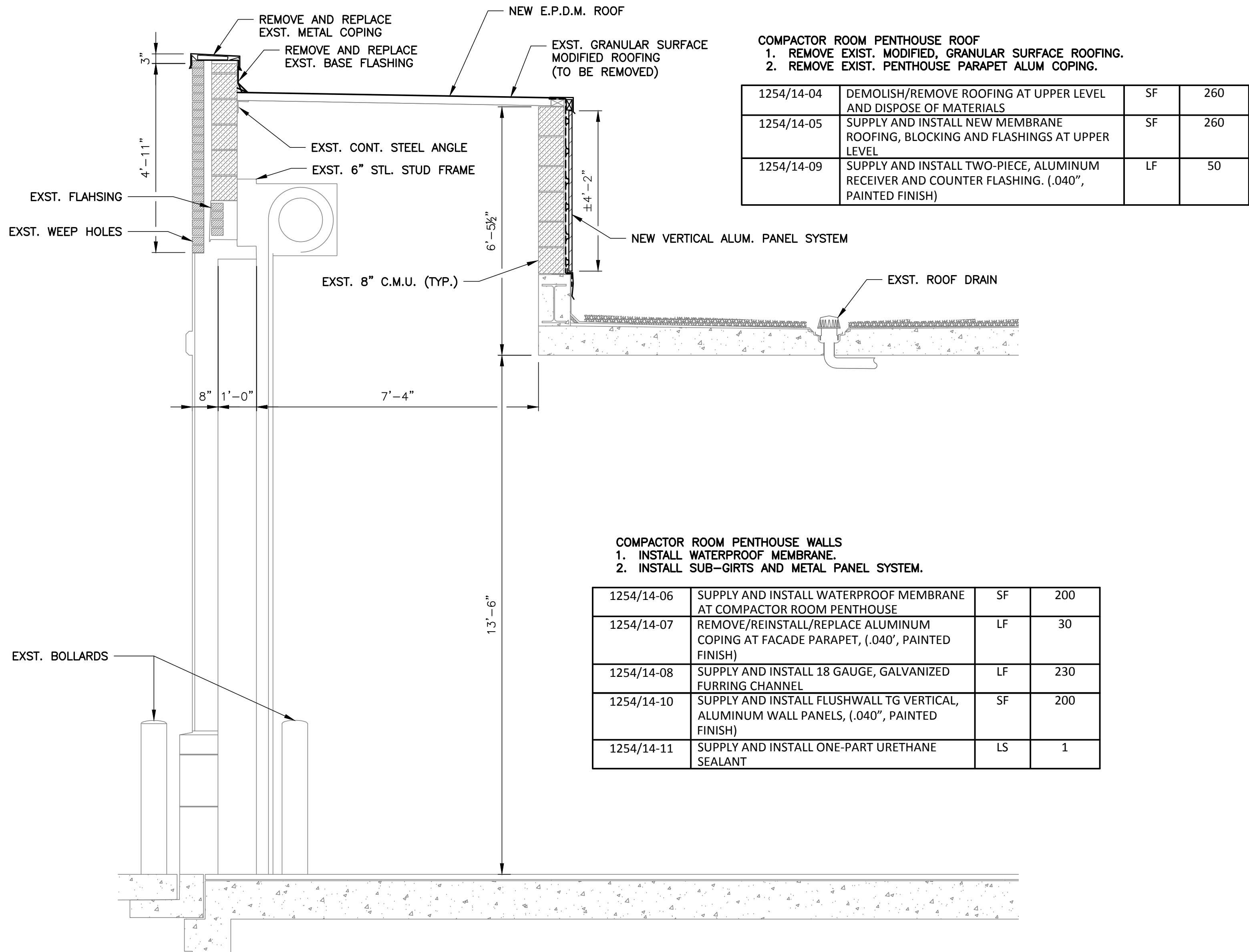
1 SECTION THRU TRASH COMPACTOR ROOM SCALE IN FEET
