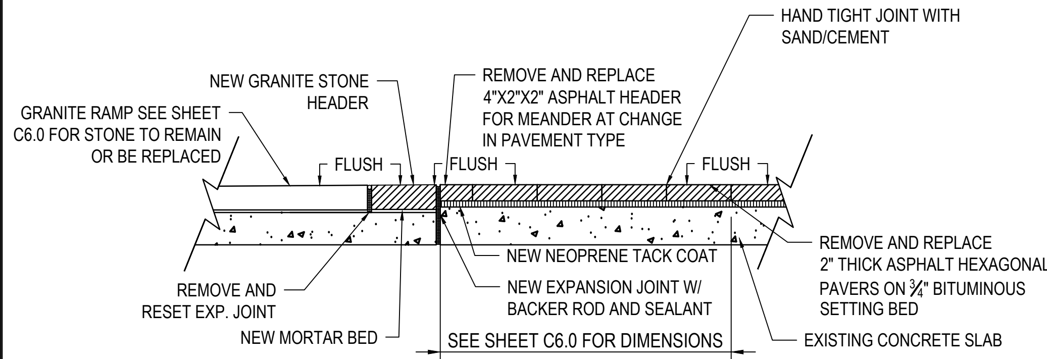
5 Ramp Header Replacement Elevation NTS
