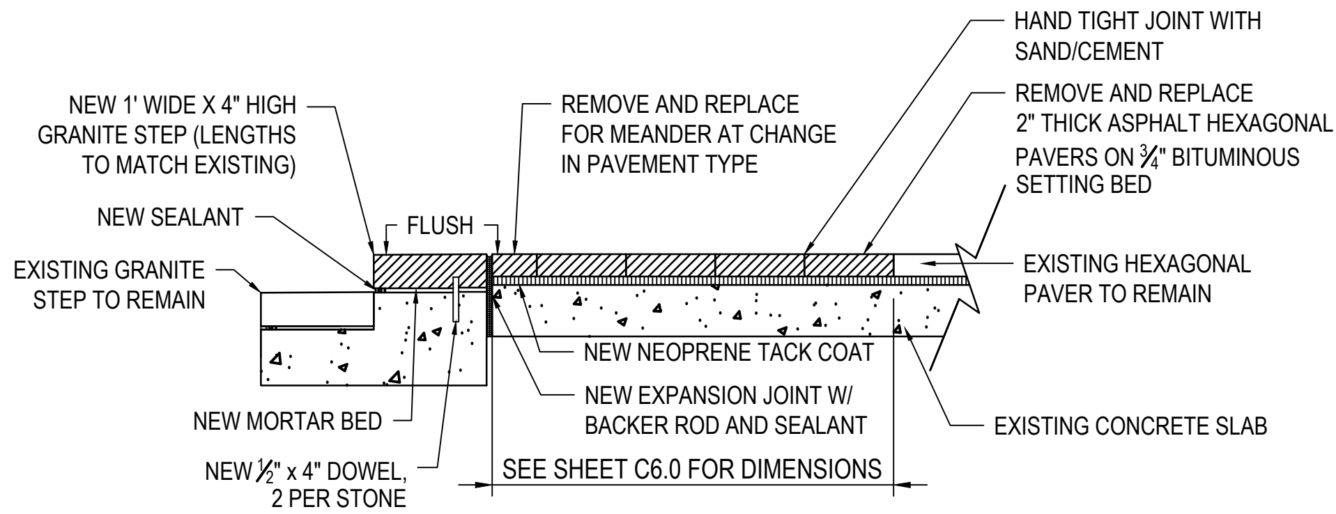
1 Step Repair Elevation NTS
