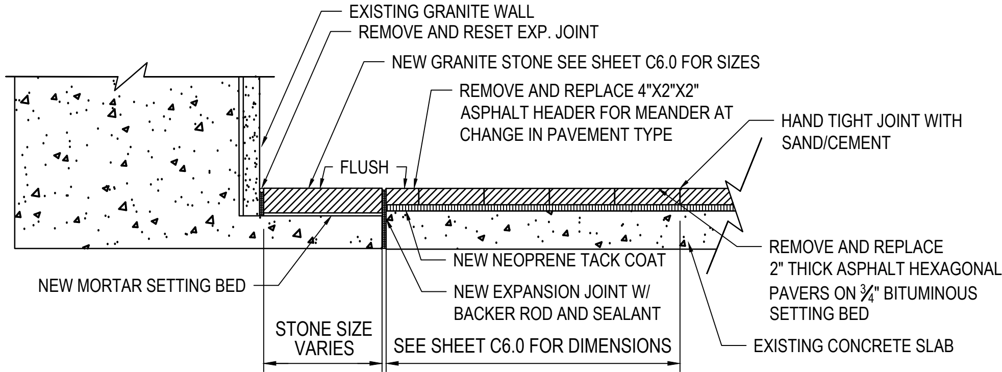
2 Landing Repair Elevation NTS
