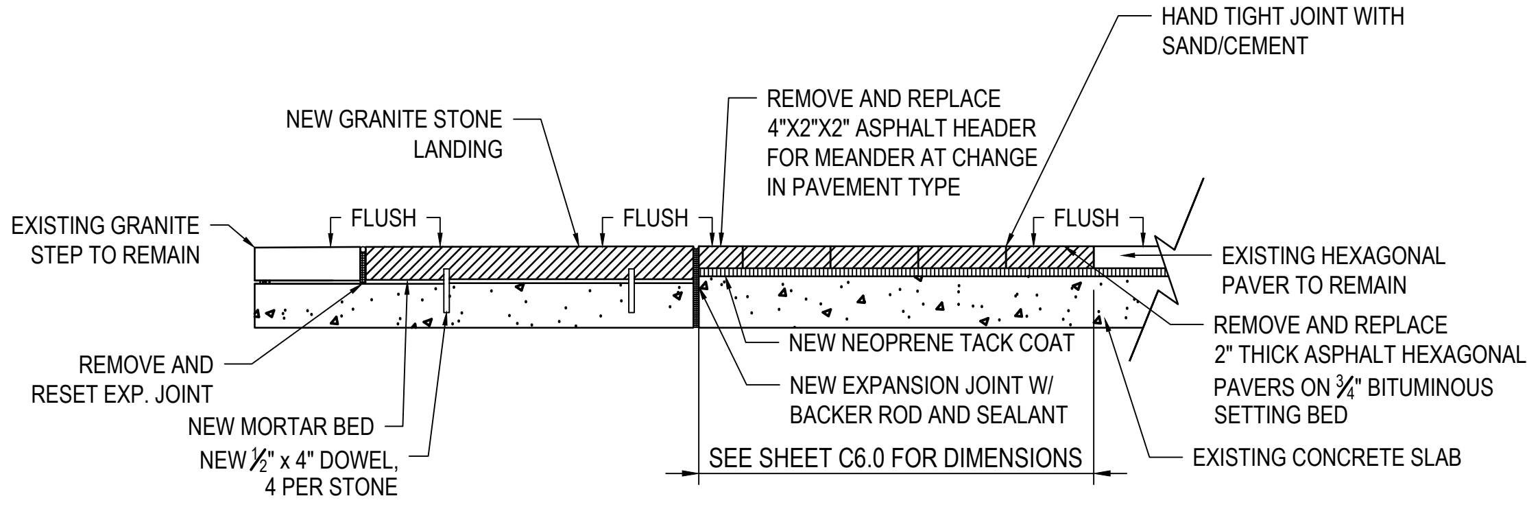
2 Landing Repair Elevation NTS
