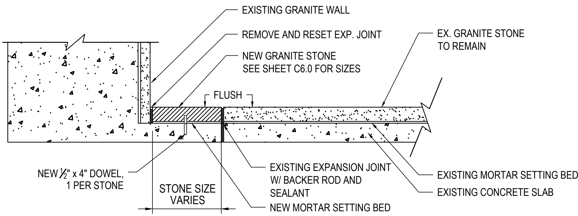
1 Step Repair Elevation NTS
