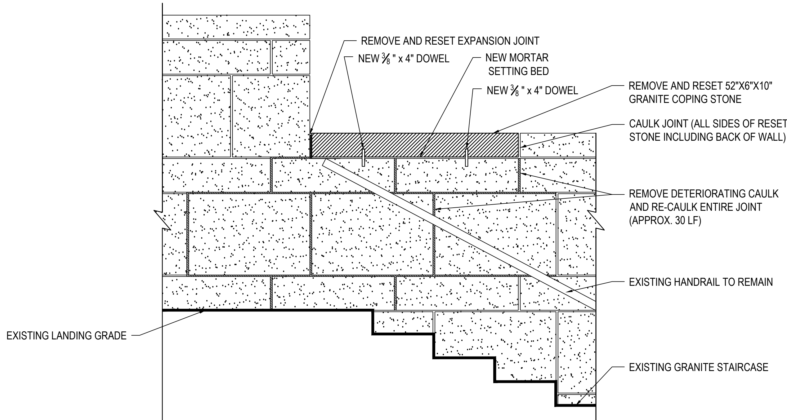
1 Wall Repair Elevation Detail NTS
