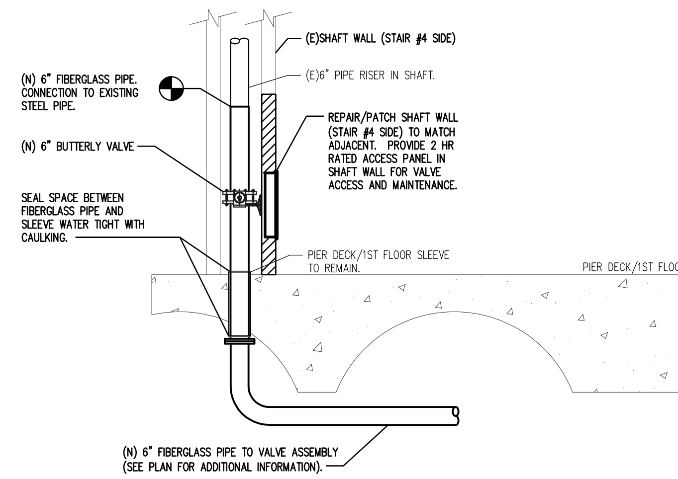
4 H-1.1 PIPE SLEEVE DETAIL - NEW WORK NTS
