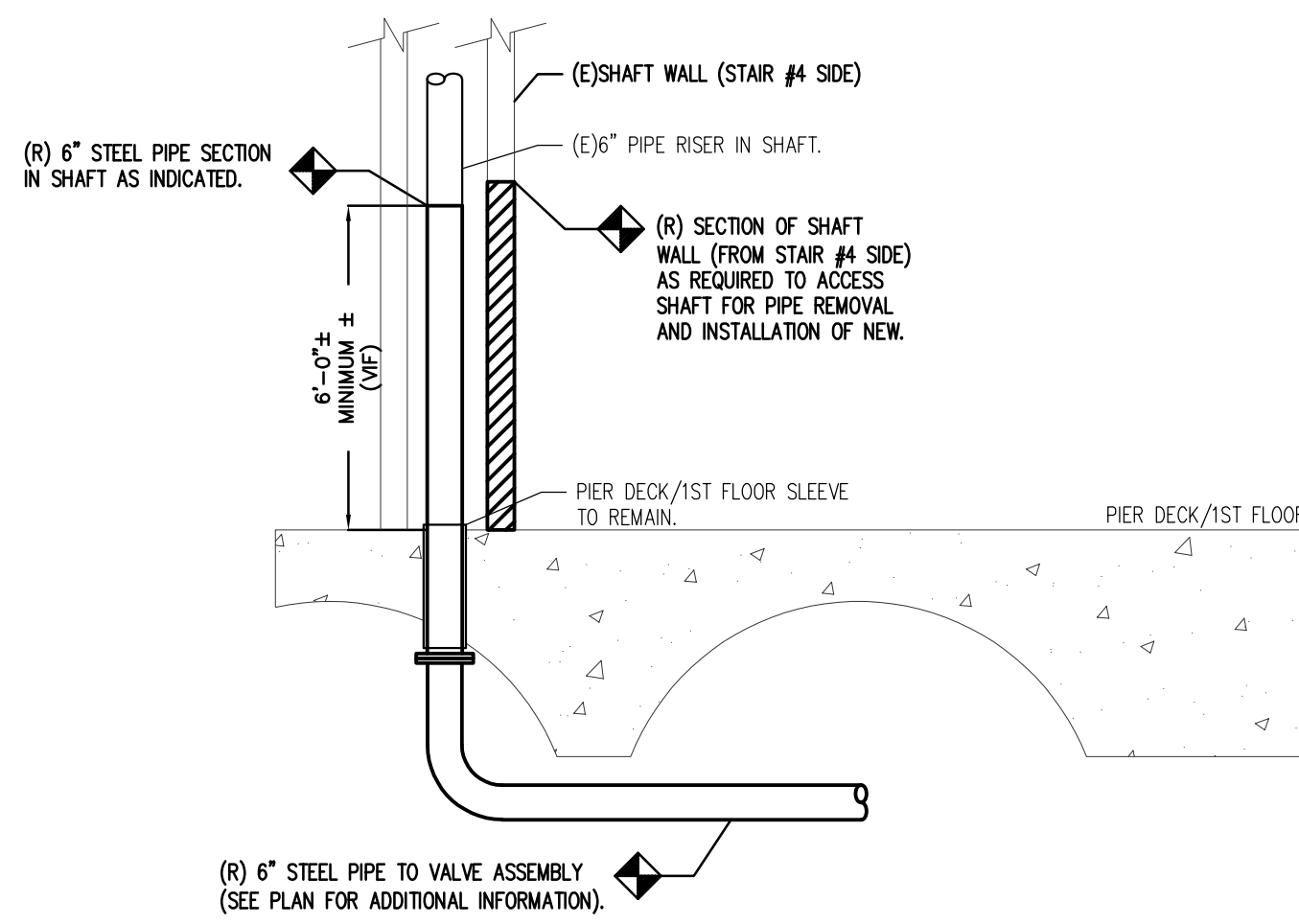
3 H-1.1 PIPE SLEEVE DETAIL - DEMOLITION NTS
