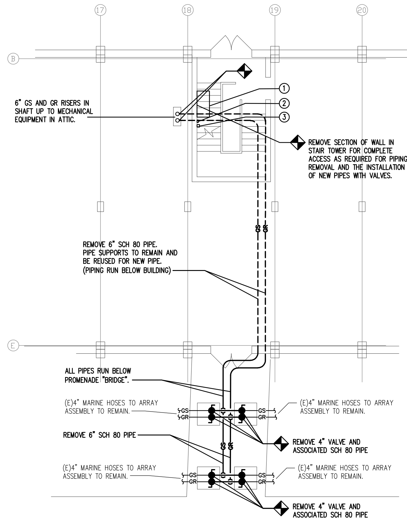
1 H-1.1 PARTIAL FIRST FLOOR PLAN - DEMOLITION 1/8"=1'-0"
