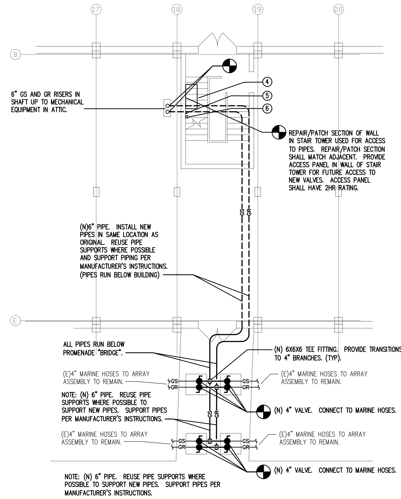
2 H-1.1 PARTIAL FIRST FLOOR PLAN - NEW WORK 1/8"=1'-0"
