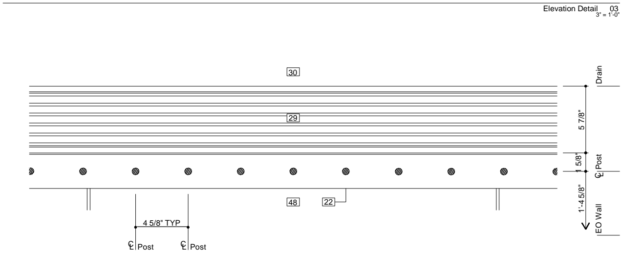
Plan Detail 02 3' = 1'-0"
